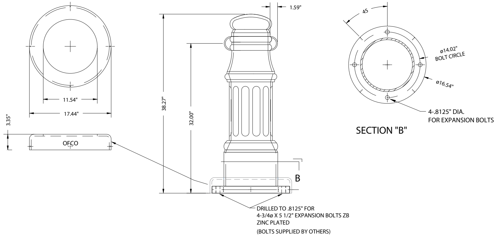
BOLLARD DETAIL
